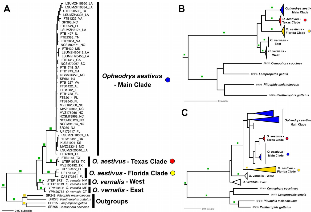
FIG. 2. (A) Bayesian maximum clade credibility phylogeny of Opheodrys aestivus based on partitioned analysis of concatenated Sanger loci. (B) Maximum likelihood phylogeny of O. aestivus from analysis of mitochondrial cytochrome b (cytb) data, partitioned by codon position. (C) Maximum likelihood phylogeny of O. aestivus based on concatenated analyses of three nuclear loci from Sanger sequence data, partitioned by locus. Symbols on nodes correspond to branch support values: green indicates Bayesian posterior probability (BPP) > 0.95 and Maximum likelihood bootstrap (MLBS) > 75, yellow indicates BPP > 0.95 and MLBS < 75. Symbols at branch tips correspond to the sampling localities in Fig. 1: yellow: peninsular Florida clade, red: central Texas clade, blue: Main clade.
