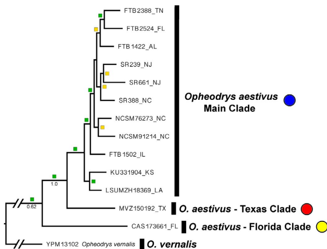
FIG. 5. Bayesian maximum clade credibility phylogeny of Opheodrys aestivus based on ddRADseq data. Symbols on nodes correspond to branch support values: green indicates Bayesian posterior probability (BPP) >0.95 and Maximum likelihood bootstrap (MLBS) >75, yellow indicates BPP >0.95 and MLBS <75. Values below branches indicate BPP support from species tree analysis of ddRADseq data in SNAPP. Colors of symbols at branch tips correspond to the sampling localities in Figs. 1 and 2.
