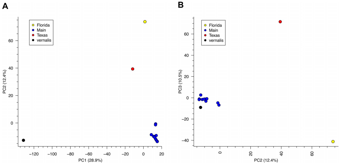
FIG. 4. Plots from principal components analysis of SNPs from ddRADseq data. (A) PC1 (28.9% of variation) vs. PC2 (12.4%), and (B) PC2 vs. PC3 (10.5%). Colors correspond to major clades as indicated in Figures 1 and 2: yellow: Florida clade, blue: Main clade, red: Texas clade, and black: O. vernalis .
