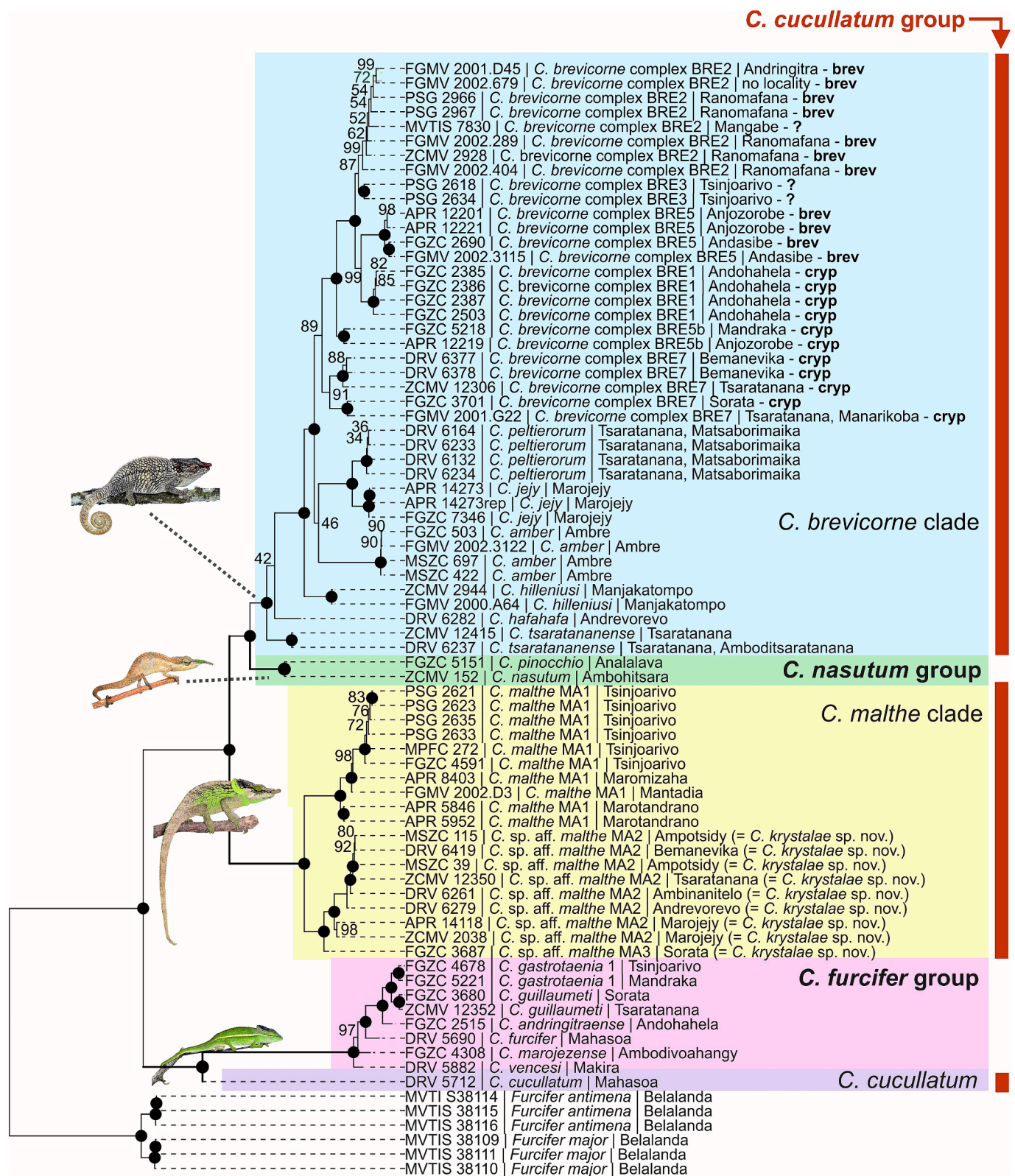
Fig. 2. Maximum Likelihood tree showing paraphyly of the informal phenetic Calumma cucullatum group of occipital-lobed chameleons, relative to representatives of the C. nasutum and C. furcifer groups. The tree is based on 77 samples and 1,643 ddRADseq loci, totalling 219,880 bp (8,135 SNPs). Black dots indicate 100% support from 1,000 replicates of ultrafast bootstraps (numbers shown where < 100%). Samples of Furcifer antimena and F. major were used as outgroups. Inset photos show representative individuals of the respective clades and species groups ( C. brevicorne , C. pinocchio , C. malthe , and C. gastrotaenia ). Vertical red bars mark the species traditionally included in the C. cucullatum group, which the tree confirms as non-monophyletic with respect to other species groups without occipital lobes. Boldface labels crp and brev in tip labels indicate tentative morphological identification of the specimens in the C. brevicorne complex.
