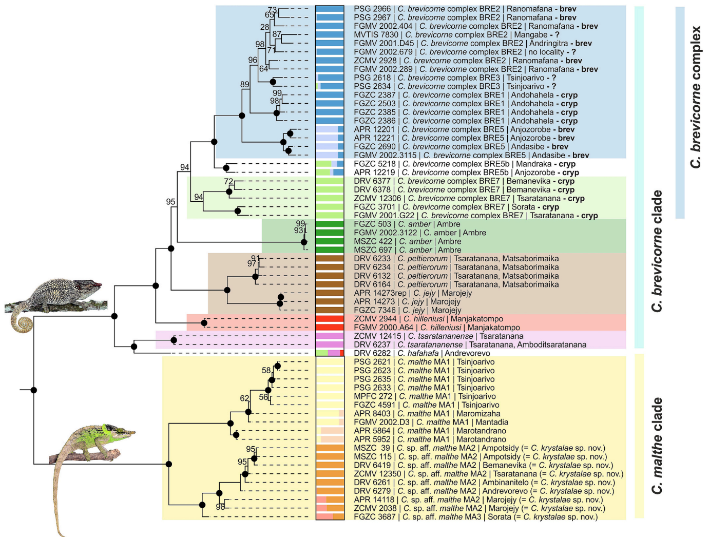
Fig. 3. Maximum Likelihood tree of 60 samples of the Calumma brevicorne clade and C. malthe clade of occipital-lobed chameleons, based on 3,546 loci derived from RADseq, totalling 480,133 bp (13,666 SNPs). The tree is rooted by C. vencesi (not shown). Black dots indicate 100% support from 1,000 replicates of ultrafast bootstraps (numbers shown where < 100%). Boldface labels cryp and brev in tip labels indicate tentative morphological identification of the specimens in the C. brevicorne complex. Barplots show assignment probabilities to the highest number of genetic clusters retrieved by Bayesian clustering with STRUCTURE, conducted separately for the C. brevicorne (3,895 SNPs, K = 7) and C. malthe clades (5,212 SNPs, K = 4). Inset photos show representative individuals of the C. brevicorne clade and the C. malthe clade (see Fig. 1).
