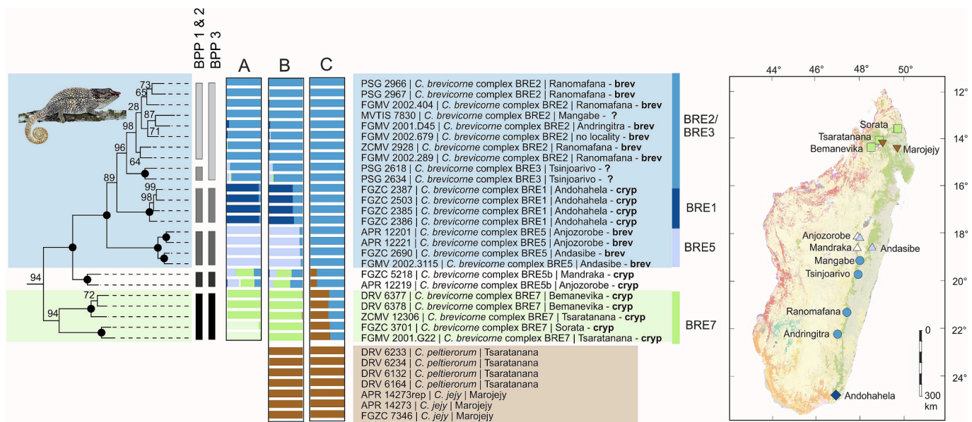
Fig. 5. Assignment of samples and clustering analysis of the C. brevicorne complex and C. peltiorum . Boldface labels cryp and brev in tip labels indicate tentative morphological identification of the respective specimens. The tree on the left shows relationships among individuals as in the phylogenomic tree in Fig. 3. Barplots show assignment probabilities to the highest number of genetic clusters retrieved by STRUCTURE for (A) samples of the C. brevicorne complex only ( K = 5 , 5,027 SNPs), (B) samples of C. brevicorne complex + C. peltiorum ( K = 5 , 211 SNPs), (C) same as B but with K = 2 . Analyses with C. peltiorum were carried out given indications for mitochondrial introgression with the C. brevicorne complex (Fig. 4). Barplots marked with BPP 1 & 2 and BPP 3 indicate the results of a lineage delimitation analysis under the multispecies coalescent, with priors on population size ( \theta ) and divergence time ( \tau ) alternative set to 0.002, (analysis 1), 0.0005 (analysis 2), and 0.02 (analysis 3). Map on the right shows geographical occurrence of the C. brevicorne complex samples included in the analysis.
