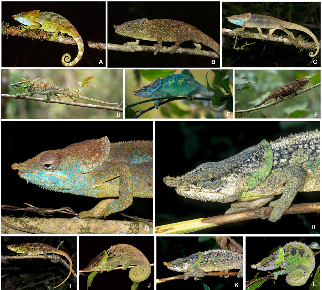
Fig. 7. Photos in life of male specimens of (A–E, G) Calumma krystalae sp. nov. and (H–L) C. malthe , and (F) one female specimen of C. krystalae sp. nov., illustrating the main morphological diagnostic differences between the two species. C. krystalae sp. nov.: (A) holotype ZSM 71/2005 from Marojejy; (B) specimen from Marojejy; (C, G) specimen from Sorata; (D) ZCMV 15202 from Marojejy; (E) uncollected male from Ampotsidy; (F) female MSZC 115 from Ampotsidy; C. malthe : (H, K, L) precise locality unknown; (I) Tsinjoarivo, (J) Maromizaha. Note uniformly sized spines in dorsal crest in the new species (vs. periodicity in size), and enlarged scales on occipital lobes (vs. scales all of similar size). All photographs by the authors.
